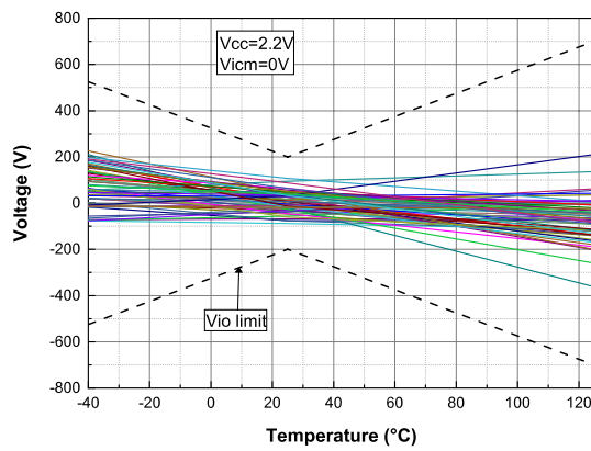
Figure 8. Input offset voltage vs. temperature at V_{CC} = 2.0\text{ V}
