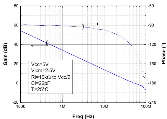
Figure 23. Open loop mode diagram at V_{CC} = 5\text{ V}
