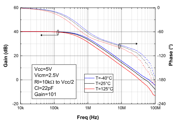
Figure 25. Closed loop mode diagram at V_{CC} = 5\text{ V}
