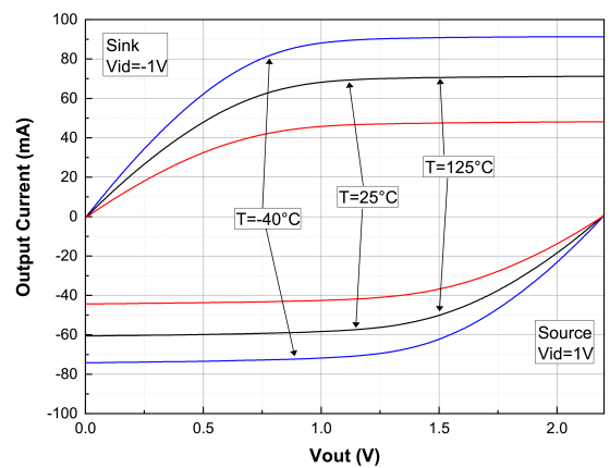
Figure 17. Output current vs. output voltage at V_{CC} = 2.0V
