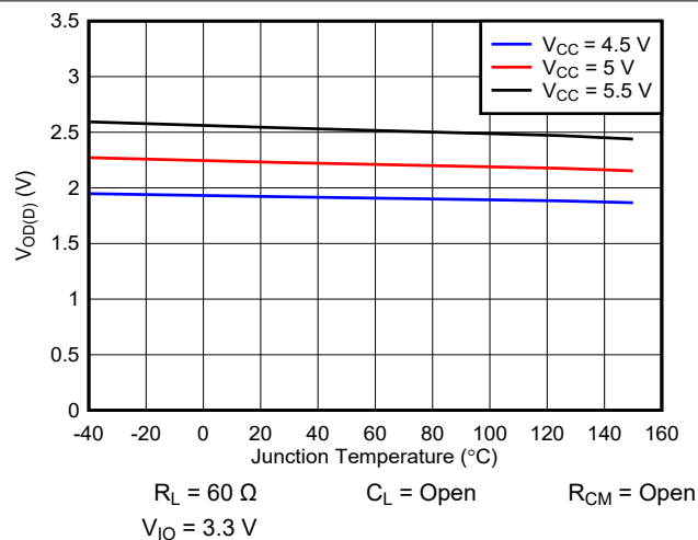
Figure 6-1. V_{OD(DOM)} vs Temperature and V_{CC}
