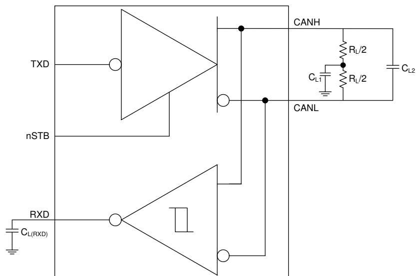
Figure 7-2. Test Circuit
