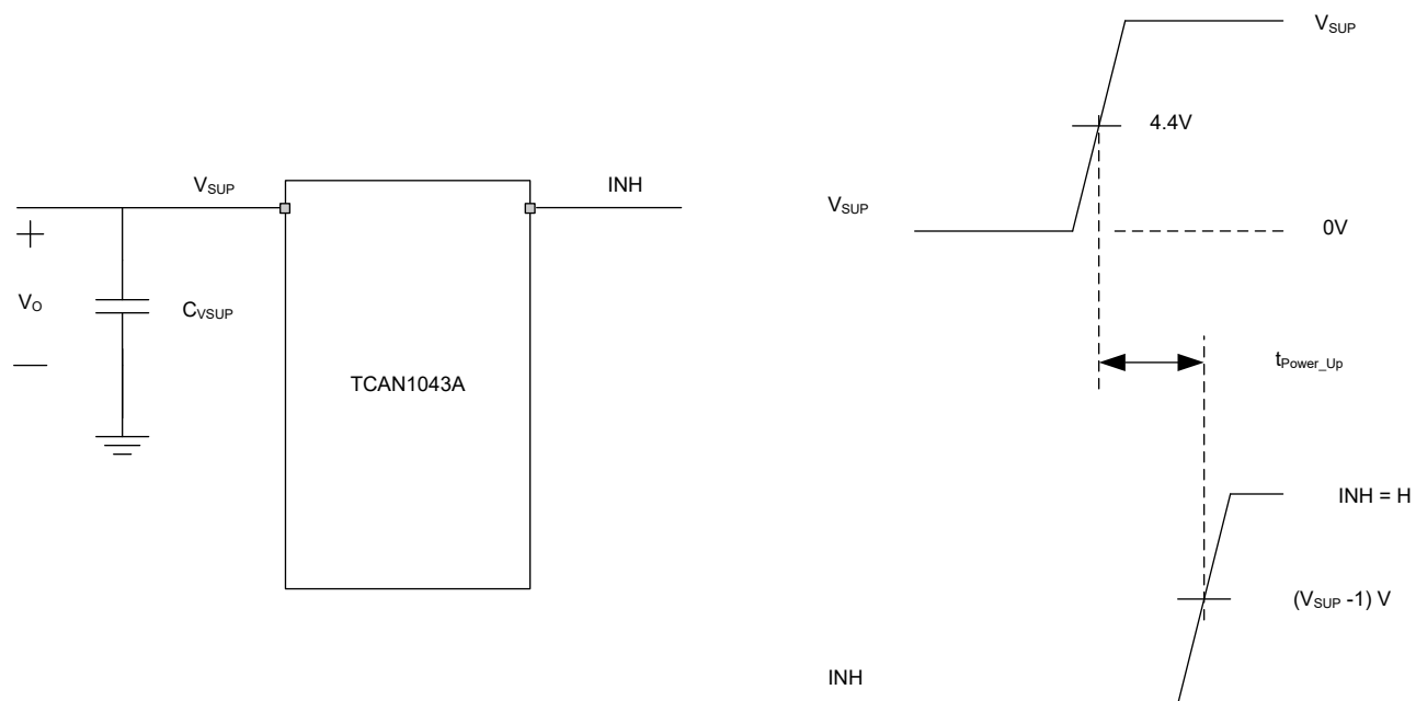
Figure 7-10. Power-Up Timing
