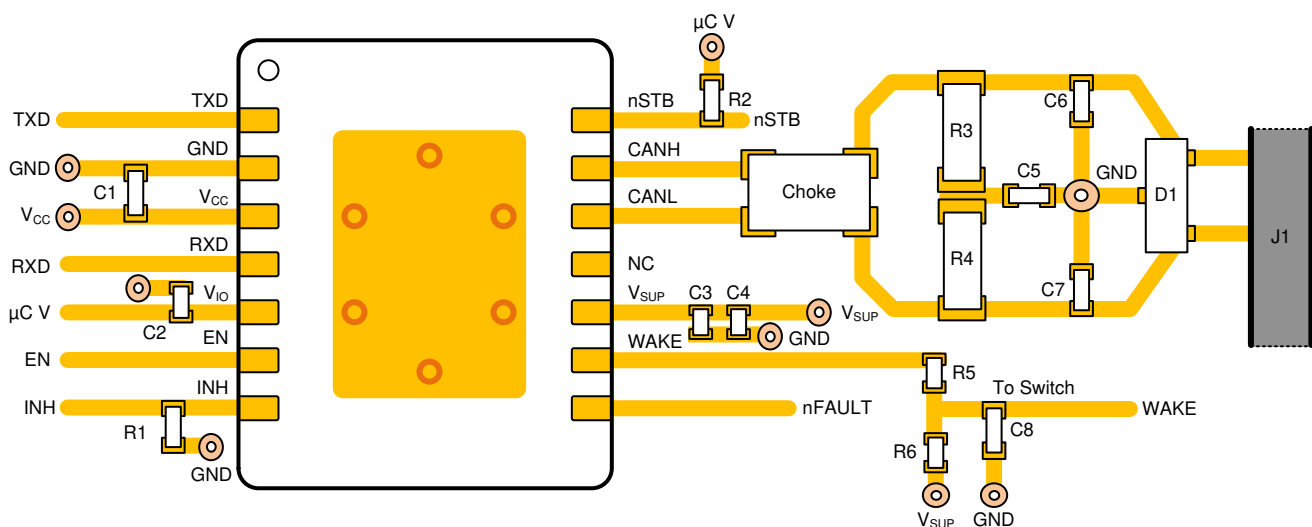
Figure 11-1. Example Layout
