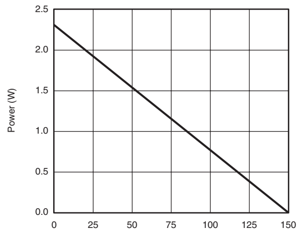
Power, Junction-to-Ambient
