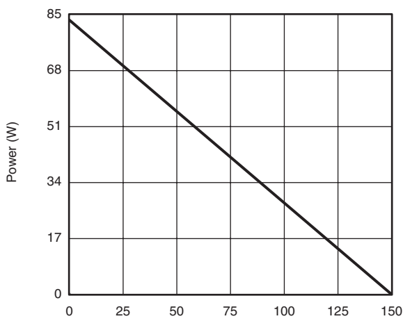
Power, Junction-to-Case
