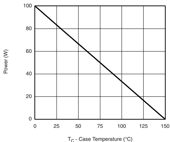
Power, Junction-to-Case
