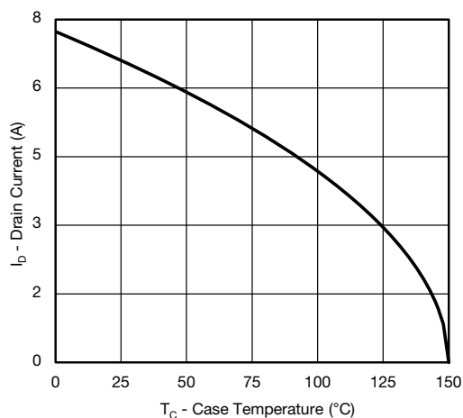
Current Derating*
