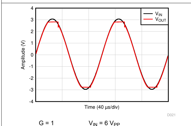
Figure 7-41. No Phase Reversal
