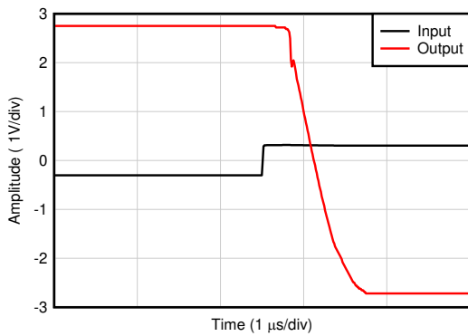
Figure 7-43. Overload Recovery
