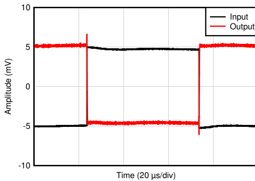
Figure 7-43. Overload Recovery
