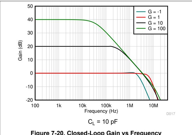
Figure 7-20. Closed-Loop Gain vs Frequency
