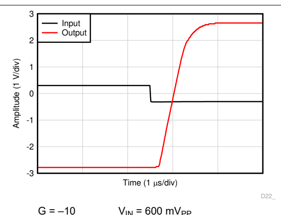
Figure 7-42. Overload Recovery
