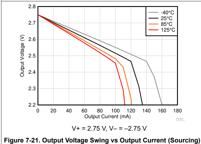
Figure 7-21. Output Voltage Swing vs Output Current (Sourcing)
