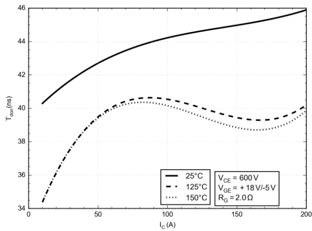
Figure 16. Typical Turn-On Switching T_{don} vs. I_C
