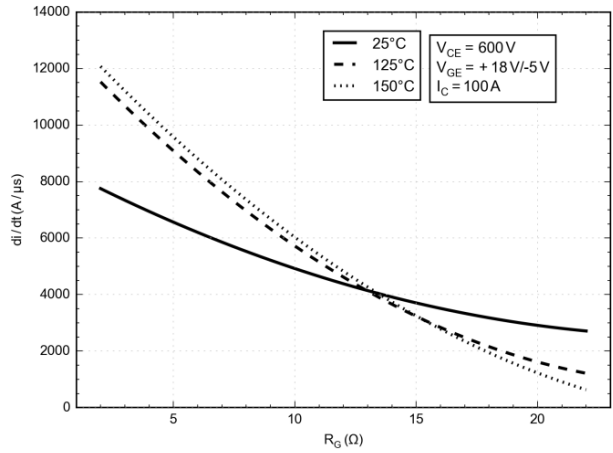
Figure 33. Typical di/dt vs. R_G
