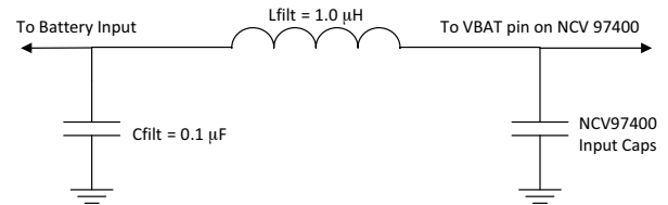
Figure 43. LC Input Filter
