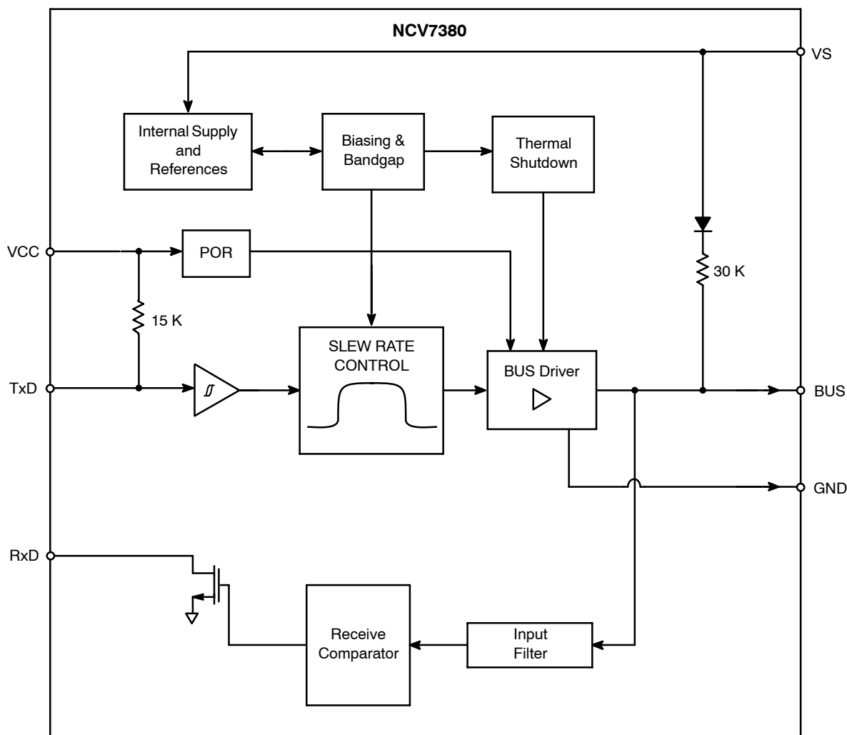
Figure 1. Block Diagram
