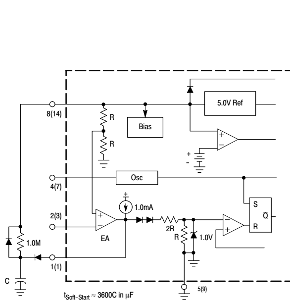
Figure 24. Soft-Start Circuit
