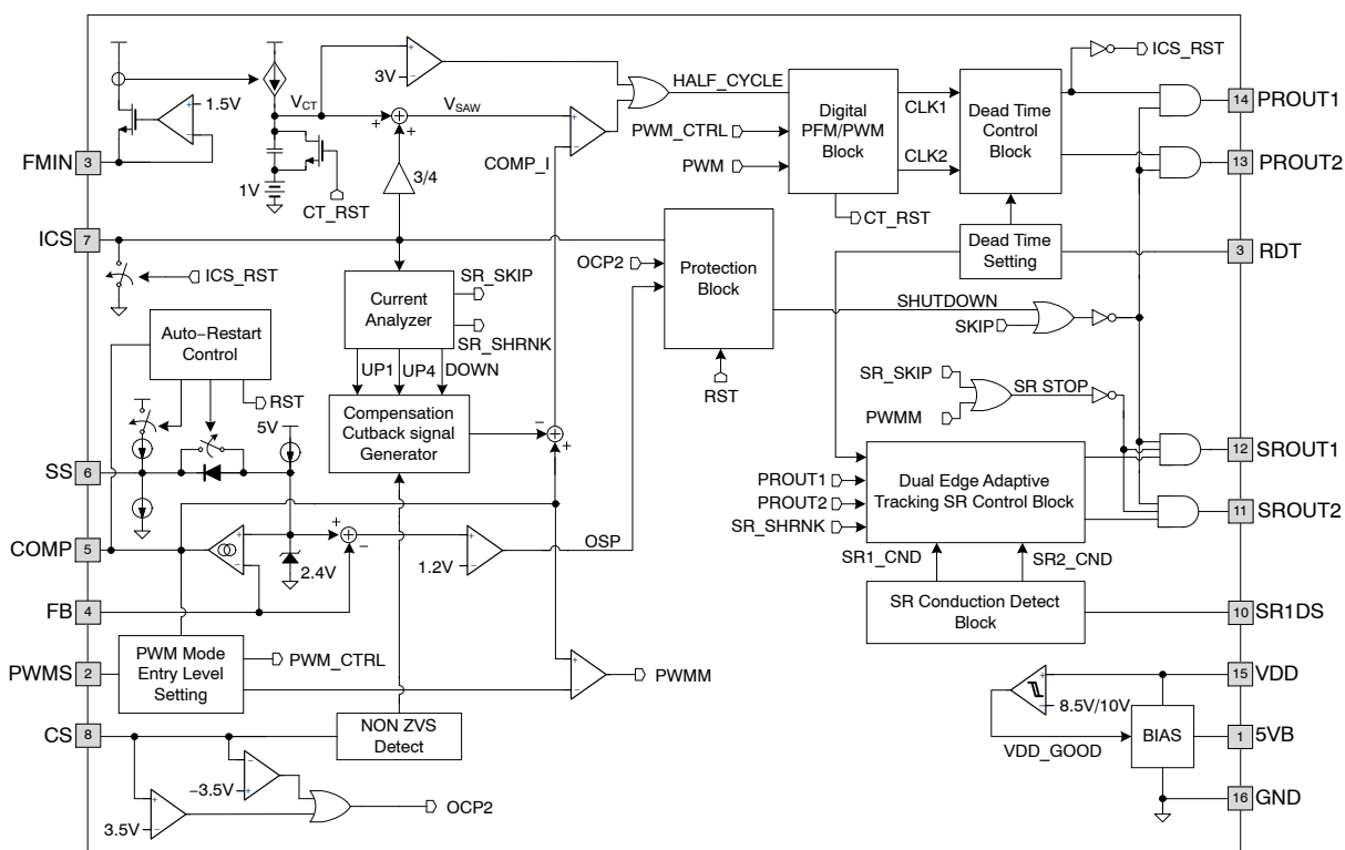
Figure 2. Internal Block Diagram of NCP4390
