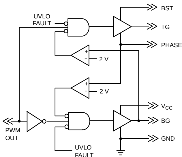
Figure 12. Block Diagram
