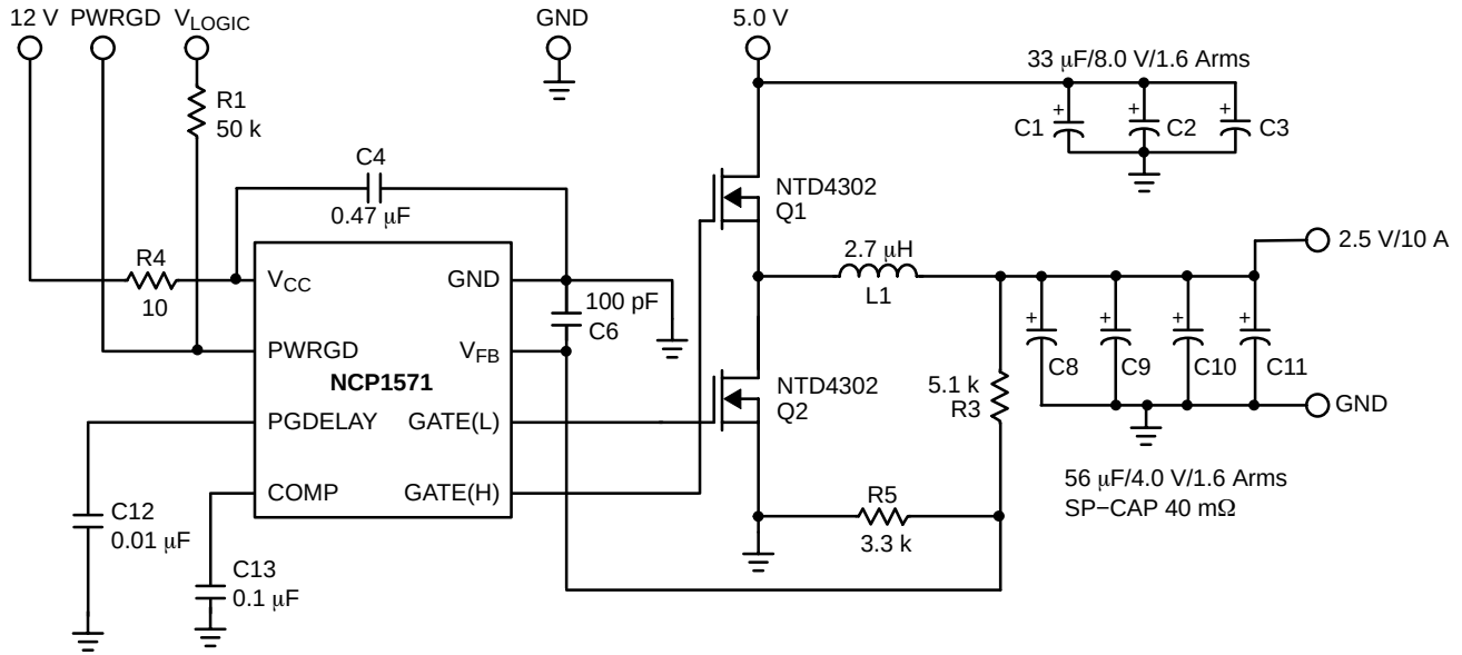
Figure 1. Applications Circuit
