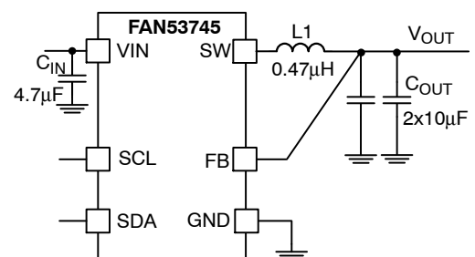
Figure 1. Typical Application
