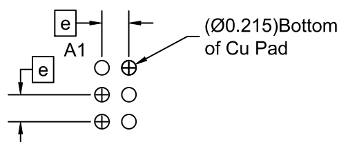
RECOMMENDED MOUNTING FOOTPRINT (NSMD PAD TYPE)
