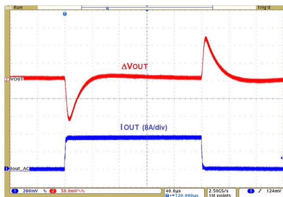
Figure 10. Load Transient 0–15 A, 10 A/\mu s
