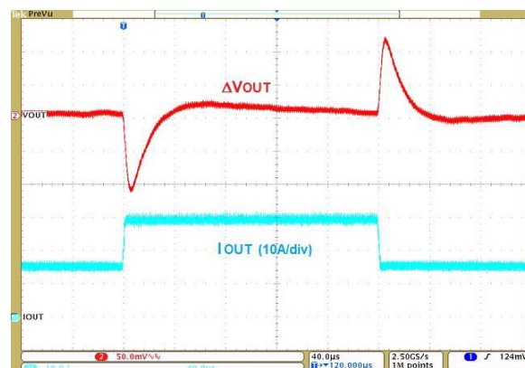
Figure 11. Load Transient 15–30 A, 10 A/\mu s
