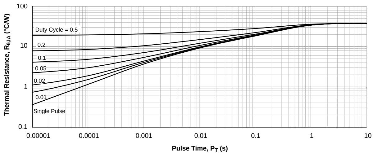
Figure 10. Thermal Response
