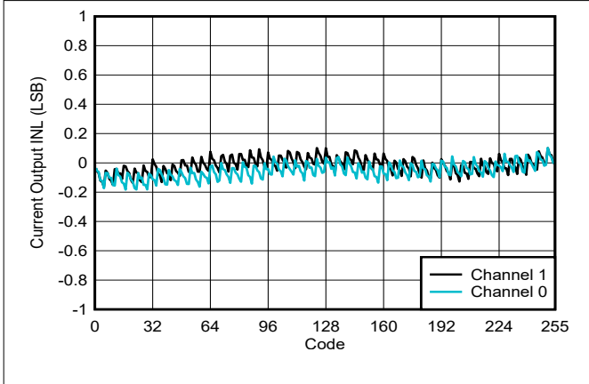
Figure 6-30. Current Output INL vs Digital Input Code
