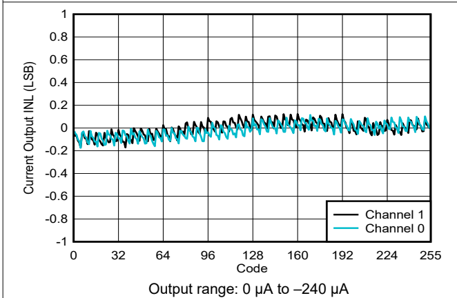
Figure 6-32. Current Output INL vs Digital Input Code
