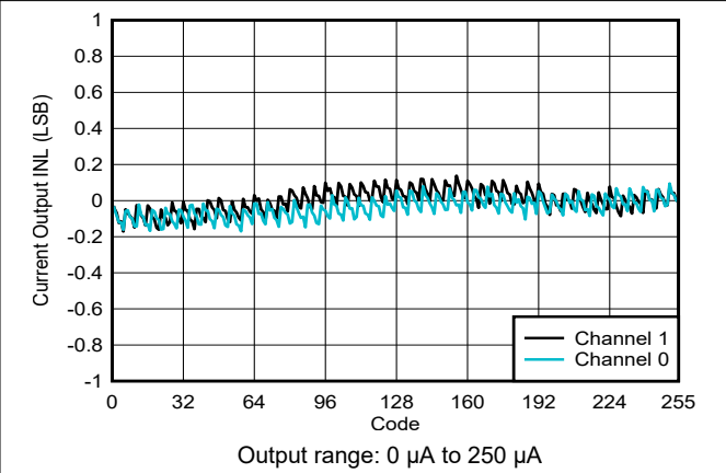
Figure 6-31. Current Output INL vs Digital Input Code
