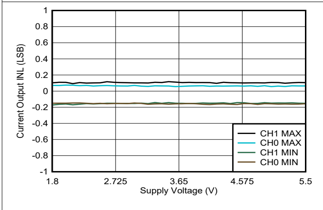
Figure 6-34. Current Output INL vs Supply Voltage
