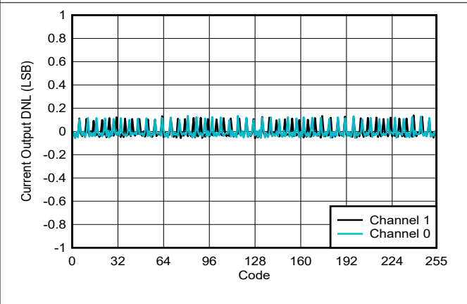
Figure 6-35. Current Output DNL vs Digital Input Code
