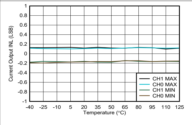
Figure 6-33. Current Output INL vs Temperature
