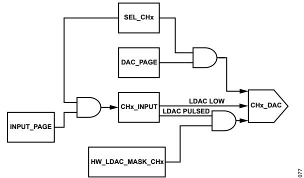
Figure 97. DAC Data Flow Between Registers
