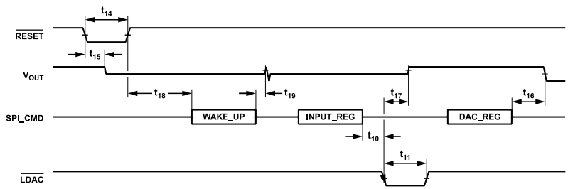
Figure 9. Start-Up Sequence Timing
