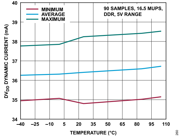
Figure 74. AD3542R-16 DV_{DD} Dynamic Current vs. Temperature
