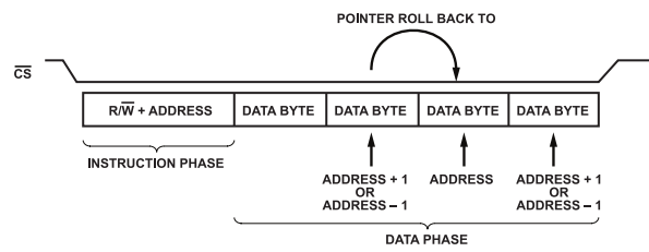
Figure 87. Looping Enabled with \text{STREAM\_MODE} = 2
